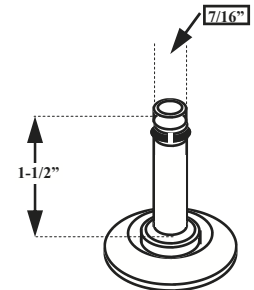
-11- GRIP RING STEM
