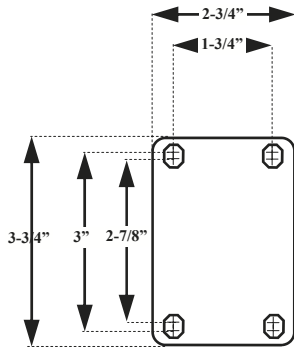
-01- TOP PLATE
