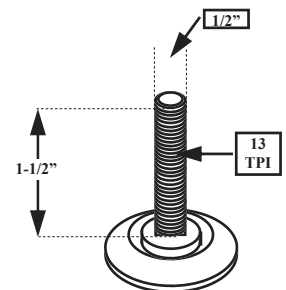
-21- THREADED STEM
