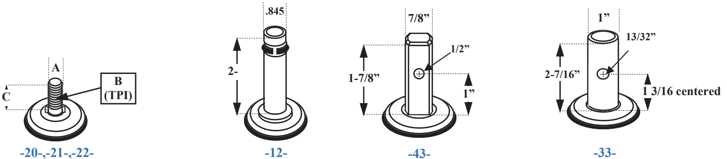
THREAD GUARDS (USE WITH BB)
